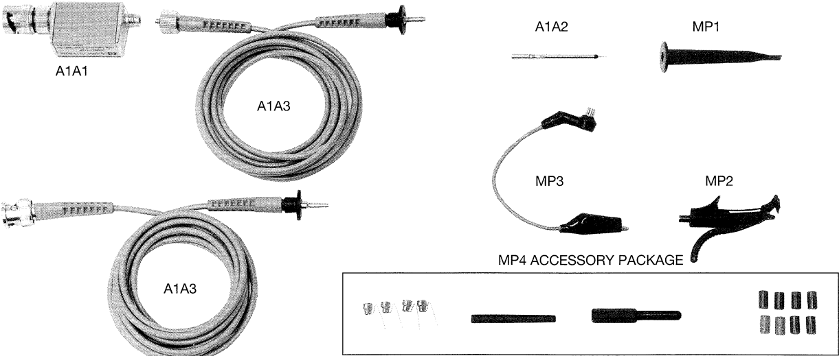
Figure 8. HP 10400A Replaceable Parts
